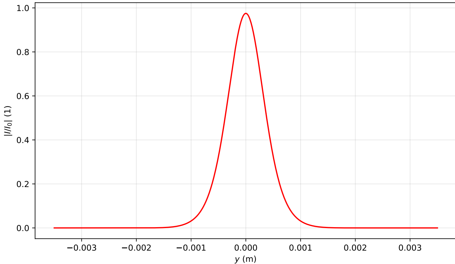
Intensity profile I(x=0, y, z=1.433)/I_0 , \text{Pin}=0.5\text{Pcr} , artificial time
